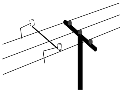
Figure 2. The proposed pantograph power pick-up mechanism
