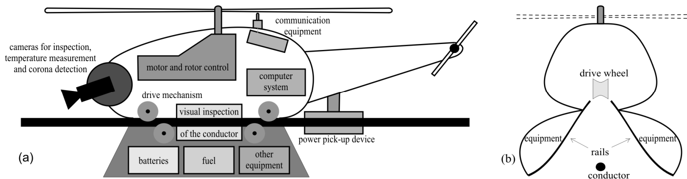
Figure 4. The proposed robot: (a) An illustration of the proposed climbing-flying robot and its components; (b) a sketch of the robot from the front, showing the rails for easier landing on conductors and equipment placement for stability.
