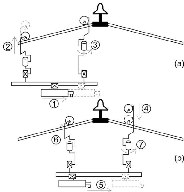
Figure 3. Obstacle traversing strategy proposed in [14].
