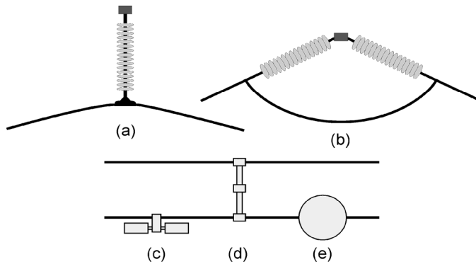
Figure 1. Obstacles on conductors: (a) suspension insulator, (b) strain insulator, (c) damper, (d) spacer and (e) aircraft warning light.
