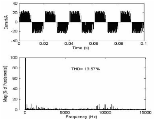
Fig.12. Input current and its spectrum analysis
