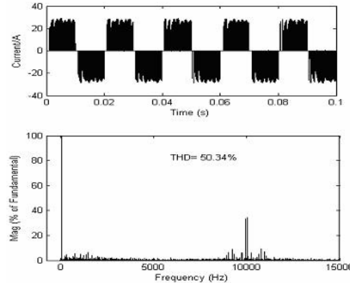
Fig.15. Input current and its spectrum analysis
