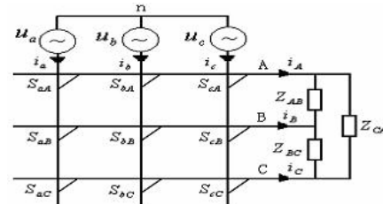
Fig. 1. The simplified topology of 3-3 matrix converter
