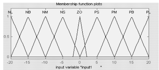
Figure 4 Membership functions for yaw error ( \epsilon )
