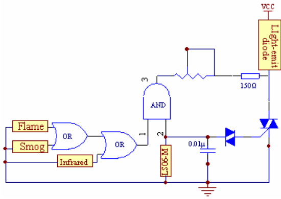
Figure 5. Circuit diagram of high-light-emitting diode
