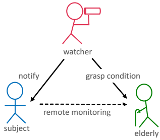
Fig. 1. Three-actor model
