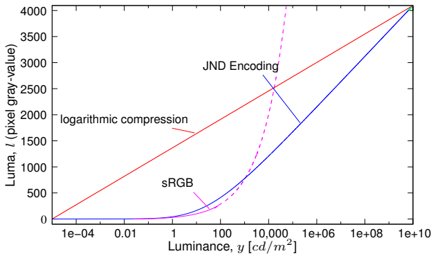
Fig. 1. Functions mapping physical luminance y to encoded luma values l . JND Encoding – perceptual encoding of luminance; sRGB – nonlinearity (gamma correction) used for the sRGB color space; logarithmic compression – logarithm of luminance, rescaled to 12-bit integer range.
