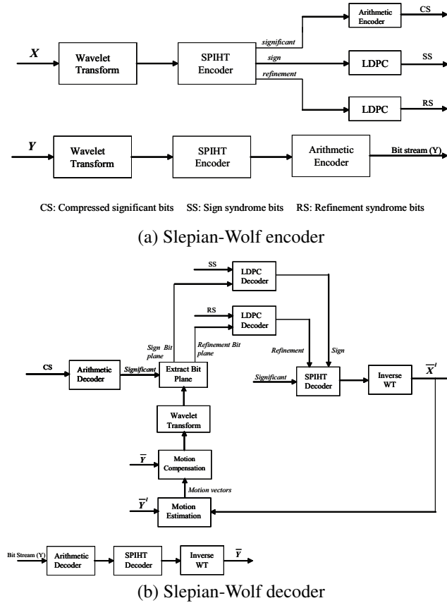
Fig. 1. Block schemes of encoders and decoder.
