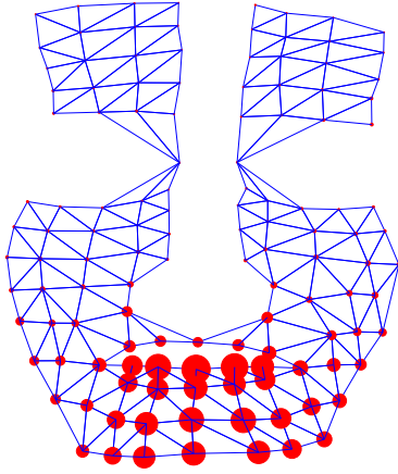
Fig. 4. Non-rigid body motion for each 3D model vertex. The circle located at each vertex describes the non-rigid body motion (high non-rigid vertex motion is equal to a big diameter of the circle).
