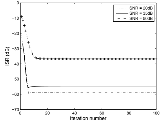
Fig. 5. Evolution of the Interference to Signal Ratio (ISR) as a function of the iteration number.
