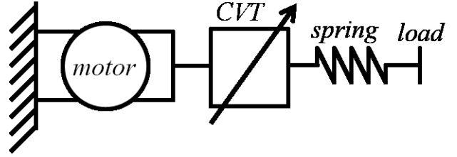
Fig. 1. The CV-SEA consists of three elements in series: an electromagnetic motor, a CVT and finally an elastic element. The series elastic element can reduce motor work, increase actuator efficiency and power, and limit motor/transmission shock, while the CVT can further optimize the speed profile of the motor for greater actuator efficiency.
