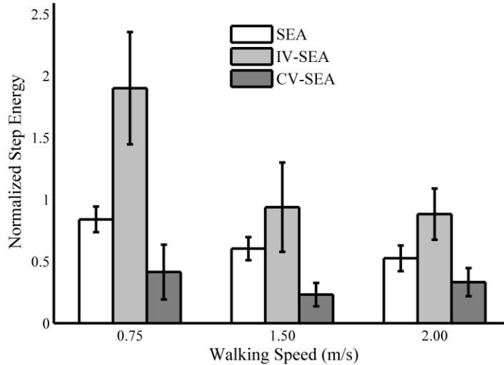
Fig. 3. The step energy of each transmission actuating a knee prosthesis was estimated for three different subjects walking at three different speeds. The step energy was normalized by the step energy required by a direct drive actuator.
