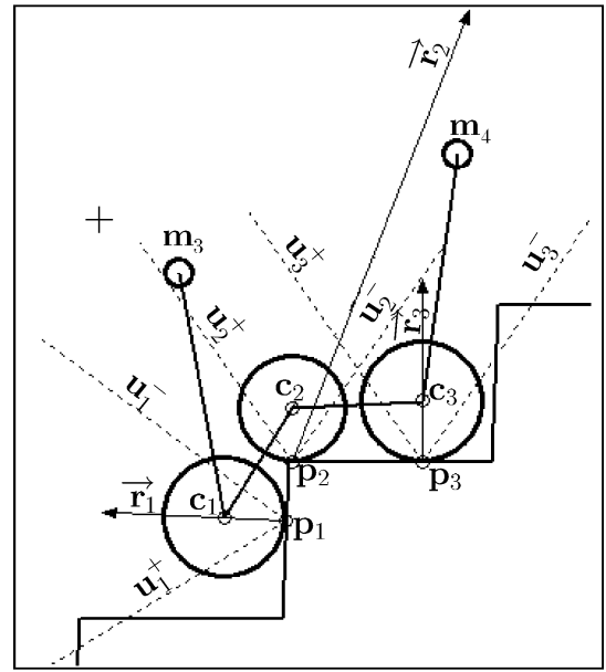
2: A configuration where the middle wheel is almost slipping. This picture has been obtained after some computations in order to be certain that the fundamental principle of static is satisfied
