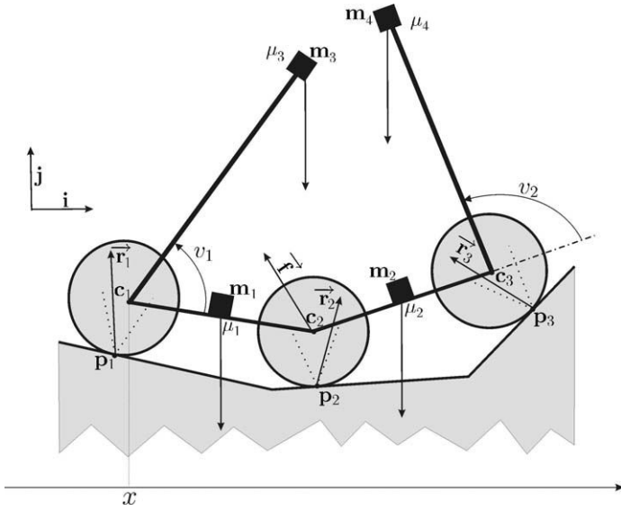
1: Two dimensional three-wheeled climbing robot to be moved in an uneven urban environment
