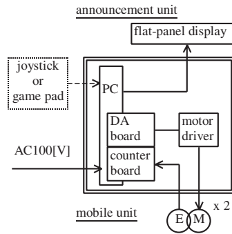
Fig. 6. System configuration of PMR-6
