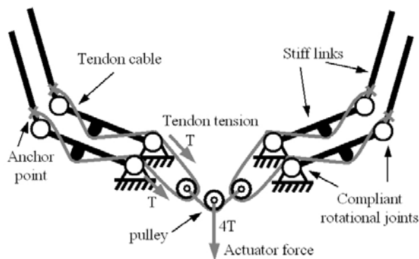
Fig. 7 Actuation schematic of the hand
