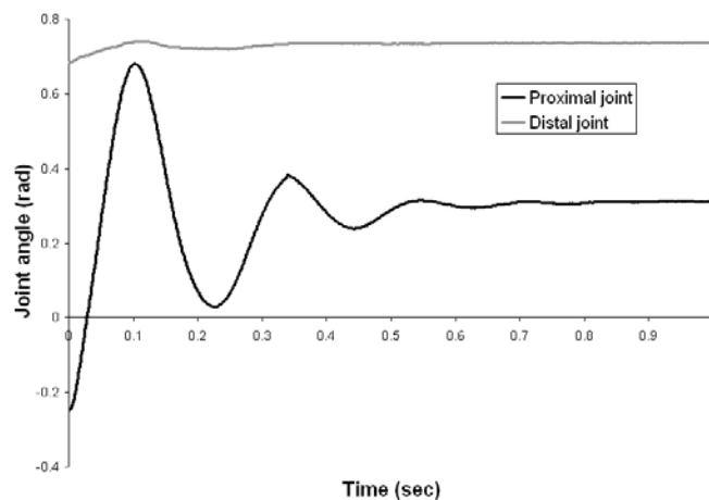
Fig. 5. Joint response of the SDM finger to a tip step displacement released at time=0.
