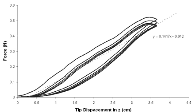
Fig. 6. Force-deflection curve of the tip of the SDM finger with linear trendline. The data represents five cycles of tip motion.
