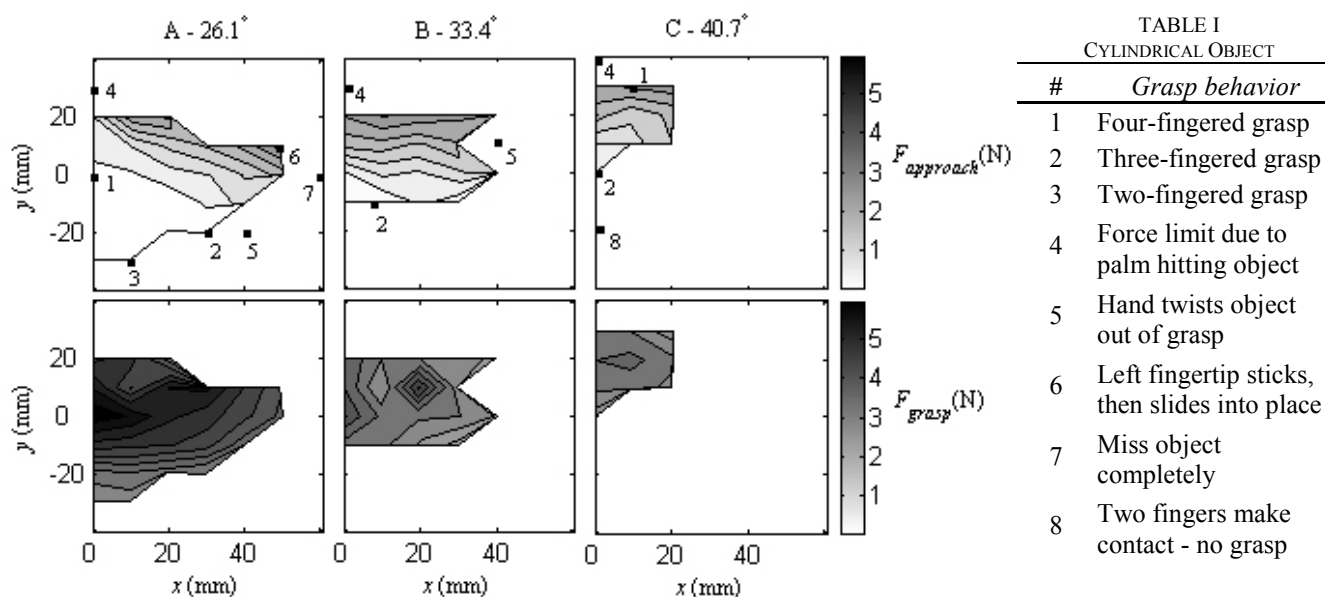
Fig. 9. Forces on the PVC cylinder object during the approach (top row) and grasp (bottom row) phases for the three object locations (columns). Labeled configurations correspond to the behavior indicated in Table I.
