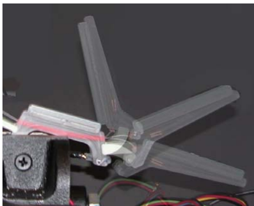
Fig. 4. Superimposed photograph of joint deflection and link motion for three positions across the travel range of the distal joint of the fingers. The center image is the rest position.
