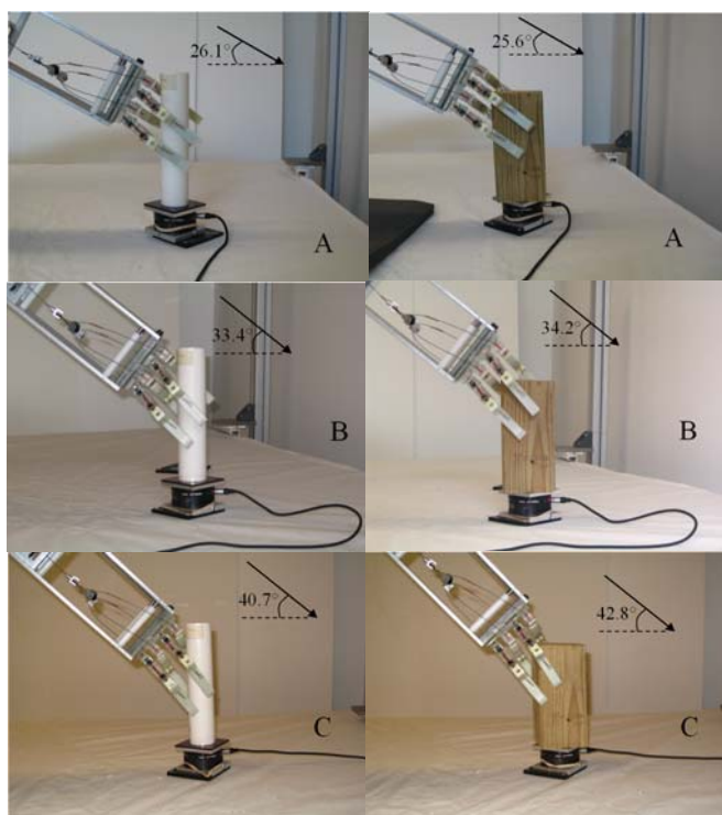
Fig. 8. Two target objects (PVC cylinder of radius 24mm and wood block with square cross-section 90mm side length) at three locations (A, B, and C). Note the differences in approach angle for the locations, the main factor affecting the force and grasp space results.
