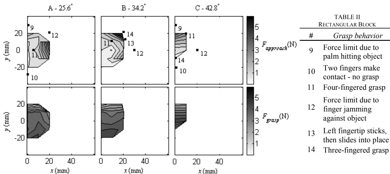
Fig. 10. Forces on the wooden block during the approach (top row) and grasp (bottom row) phases for the three object locations (columns). Labeled configurations correspond to the behavior indicated in Table II.
