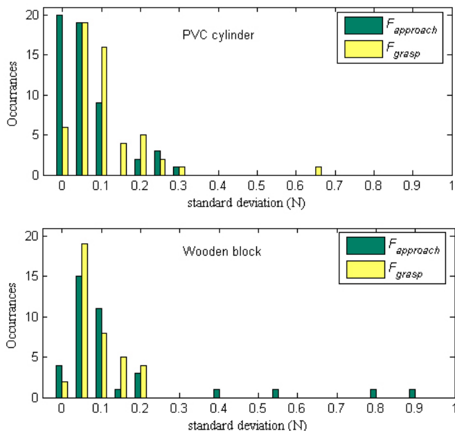
Fig. 11. Histograms of the standard deviation of the force measurements for the PVC cylinder (top) and wooden block (bottom).
