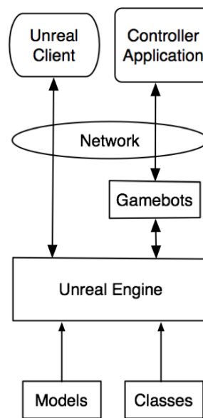
Fig. 1. USARSim's architecture
