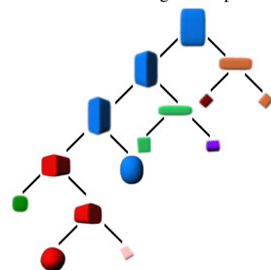
Fig. 1. A decomposition tree, with n=8 . The leaf nodes are merged pairwise to form a binary tree from the bottom up. Note to readers: figures should be viewed in color.
