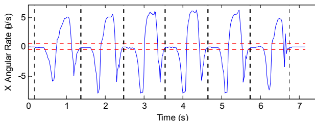
Figure 6. Foot angular rate in the ankle axis.
