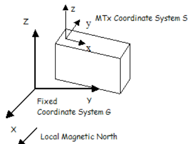
Fig. 3. Earth-Fixed Coordinate frame and Acceleration Sensor Coordinate frame
