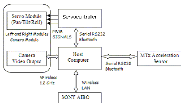
Fig. 5. Block Diagram. Ocular Servo Module receives input from Servocontroller SSC-32 (Lynxmotion® Technologies) and Host Computer. Communication channels with various peripheral modules are shown.
