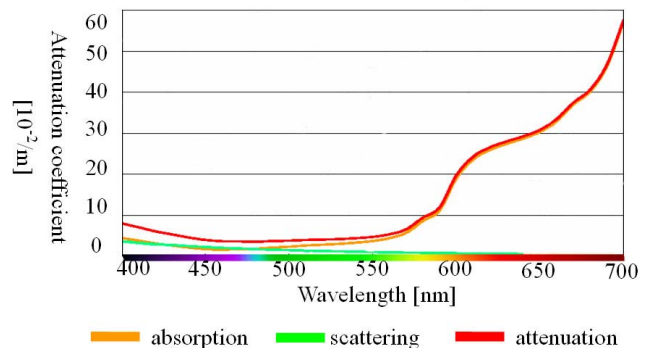
Fig. 5. Attenuation coefficient of water.
