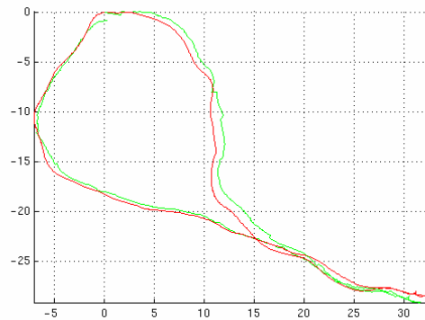
Figure 8 Top: Frame system of an extended outdoor run. Global pose from GPS and inertial sensors (green), frame system in blue. Note the overshoot at the end of the loop. Bottom: Frame system with loop closure, in red.
