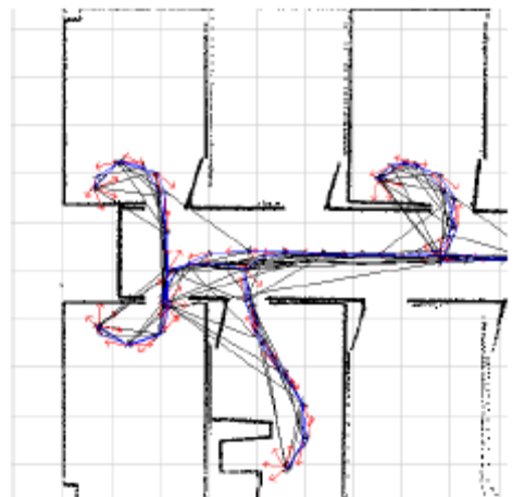
Figure 1 Frames linked by matching laser scans. Red arrows are frames, lines are links. Whenever there is a significant overlap of scans, a link is inserted, e.g., when the LRF sees through a doorway into the hall from separate rooms.
