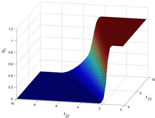
Fig. 8: Representation of \eta_1 as a function of r_{13} and r_{23} .
