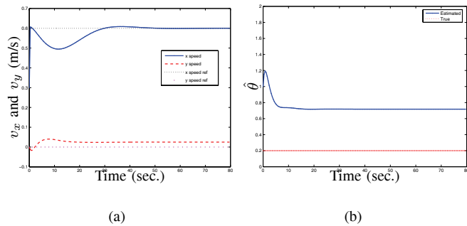
Fig. 7. Simulation results. (a) Robot velocity in the body-fixed frame, and (b) the estimated friction parameter.
