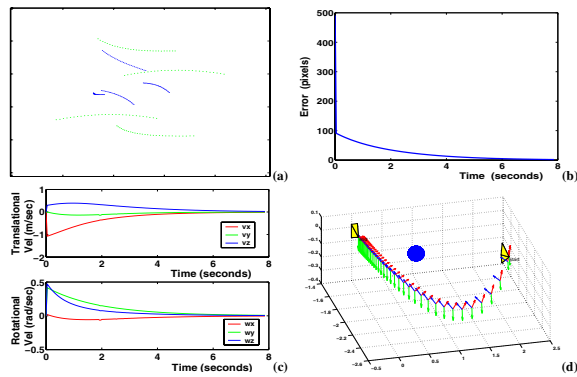
Fig. 8. Simulation Result: (a) Initial (blue) and Desired (green) images (b) Smooth convergence of Error Norm (c) Stable Velocity Screw (d) Camera Trajectory
