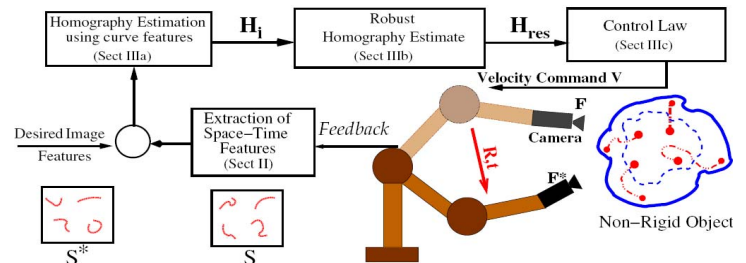
Fig. 1. Proposed scheme for visual servoing in non-rigid environments
