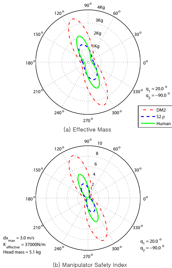
Fig. 9. (a) Effective mass of DM^2 , S2\rho and Human at q_1 = 20^\circ and q_2 = -90^\circ . S2\rho has a maximum effective mass of 1.4kg as compared to 3.5kg for DM^2 and 2.2kg for Human, while conventional PUMA560 has an effective mass of 25kg. (b) The Manipulator Safety Index (MSI) of DM^2 , S2\rho and Human at the same configuration. When the MSI or equivalent HIC_{15} is less than 10, the probability of minor brain injury is zero. [1]
