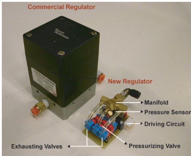
Fig. 3. The newly designed regulator is more compact than a commercial one. It consists of four parts: pressure sensor, solenoid valve, manifold and driving circuit.
