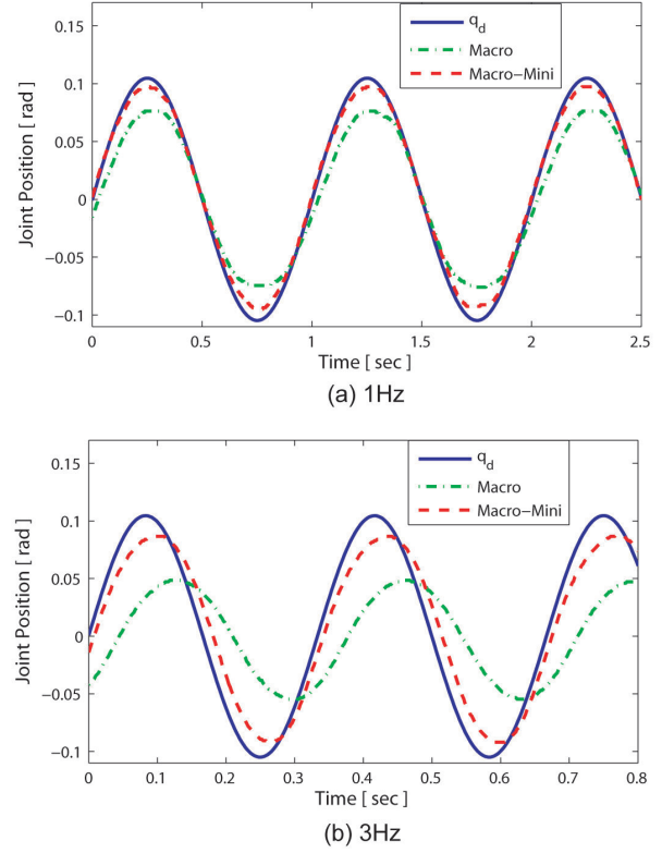
Fig. 8. Comparison of position tracking performance for pneumatic muscle actuation (Macro) and hybrid actuation (Macro-Mini) at 1 Hz and 3 Hz. (a) The result shows that the hybrid actuation is five times faster than the pneumatic muscle actuation alone. (b) The hybrid actuation is able to track the trajectory with a small error, while the pneumatic muscle actuation alone shows significant phase and amplitude distortion.
