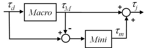
Fig. 7. Block diagram of Hybrid Actuation Control. The macro is an antagonistic pair of pneumatic muscles, the mini is an electrical motor.
