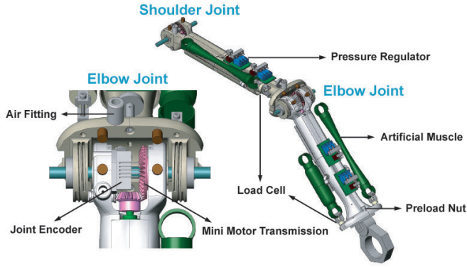
Fig. 6. Detailed view of the Stanford Human Safety Robot with a hybrid actuation approach.
