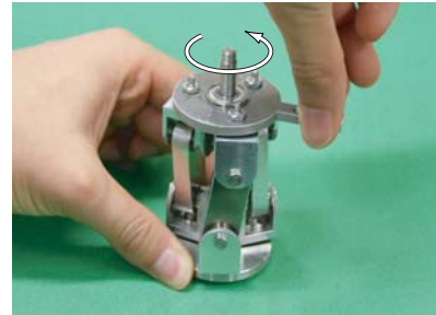
Fig. 4. Twist motion of the designed mechanism
