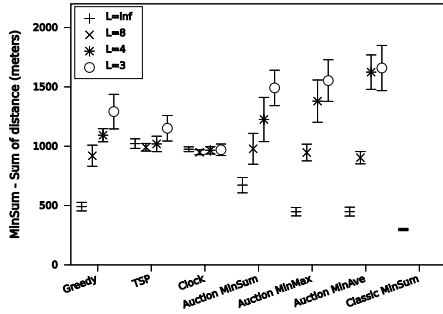
Fig. 5. Total distances traveled by all robots for each algorithm. Mean values and the 95% confidence intervals are shown in each case.
