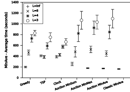
Fig. 7. Average task completion time for each algorithm. Mean values and the 95% confidence intervals are shown in each case.
