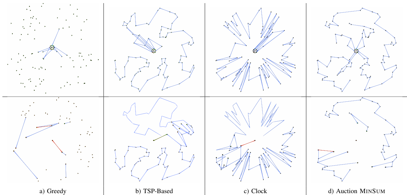
Fig. 4. Two snapshots of each algorithm in action, at initial (top) and intermediate (bottom) mission execution. Lines indicate task ordering.
