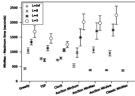
Fig. 6. Total mission completion time for each algorithm. Mean values and the 95% confidence intervals are shown in each case.
