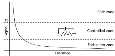
Fig. 3. Typical degradation of the radio signal quality as a function of the distance between transmitter and receiver. When quality falls below a safety threshold ( st ), a spring is activated to prevent network disconnection.
