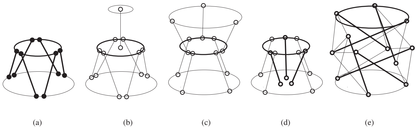
Fig. 8. Legs in thick lines correspond to rigid bars, while those in thin lines correspond to elastic tendons.
