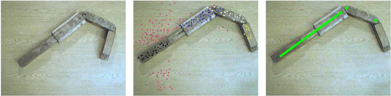
Fig. 7. Experimental results showing the extraction of the kinematic properties of a wooden toy (length: 90cm) using interactive perception. The left image shows the object in its initial pose. The middle image shows the object after the interaction. The detected clusters corresponding to rigid bodies are displayed. The right image shows the detected kinematic structure (green line marks the prismatic joint, green dots mark the revolute joints).
