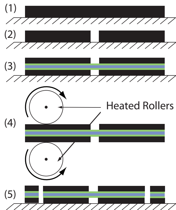
Fig. 4. A step-by-step illustration of the posterboard link and hinge fabrication process
