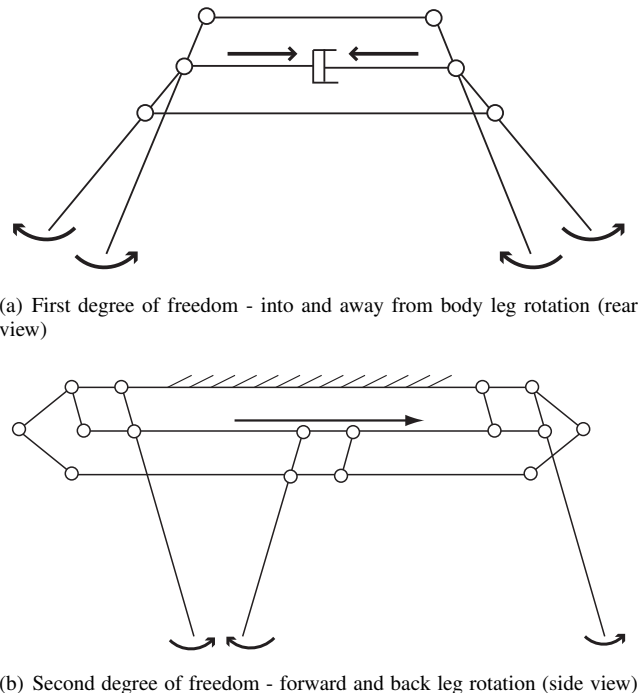
Fig. 5. Prototype crawler kinematics showing two independent degrees of freedom
