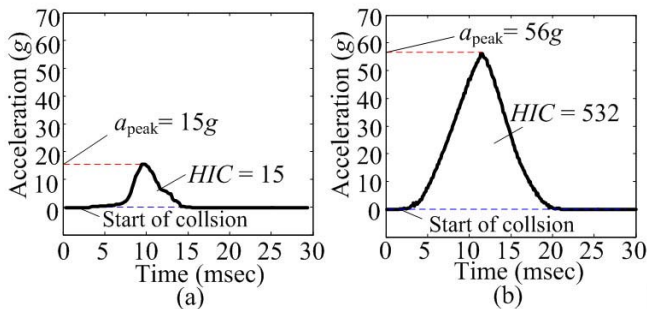
Fig. 13 Experimental results for dynamic collision of robot arm; acceleration versus time (a) with SJM, and (b) without SJM.
