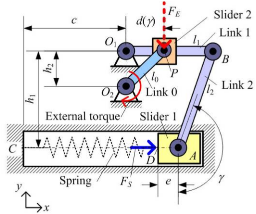
Fig. 3 Slider-crank mechanism combined with spring.
