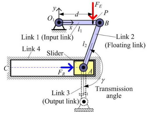
Fig. 2 Slider-crank mechanism.
