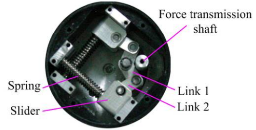
Fig. 10 Prototype of SJM.
