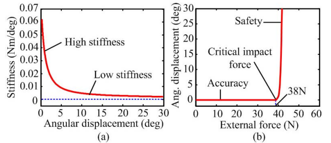
Fig. 6 Analysis of slider-crank mechanism combined with spring; (a) equivalent stiffness of SJM as a function of angular displacement, and (b) angular displacement versus external force.
