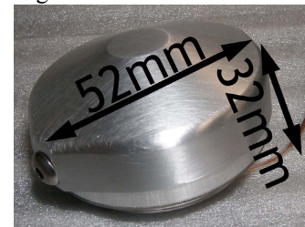
Fig. 3. 5 Nm-Class CMRFB
