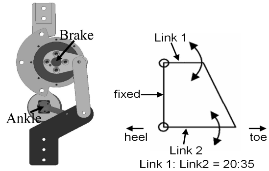
Fig. 5. Linkage Mechanism
