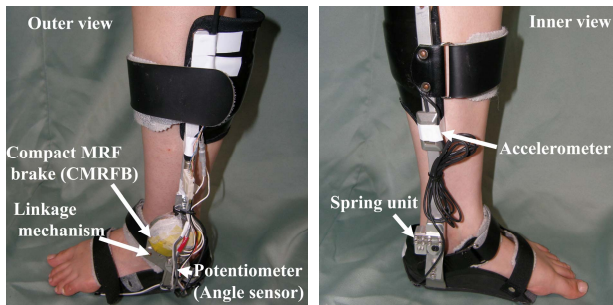
Fig. 2. Third-generation i-AFO with 5 Nm-class CMRFB
