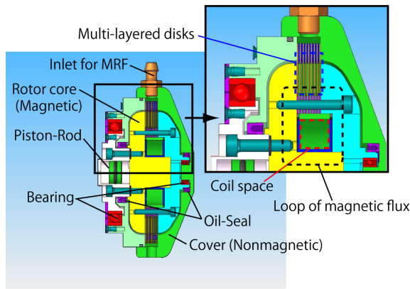
Fig. 4. Cross-section of the 5 Nm-class CMRFB
