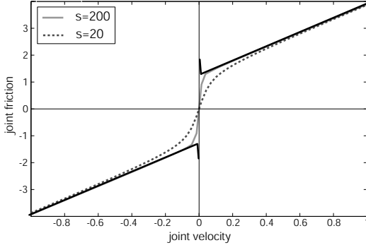
Fig. 3. Approximative continuous friction model. Solid black line represents the theoretical discontinuous Coulomb friction. For an (example) steepness parameter of s = 200 the derivatives at the start condition ( \dot{\mathbf{q}} = 0 ) become too large and ILQG diverges whereas for s = 20 it successfully converges.
