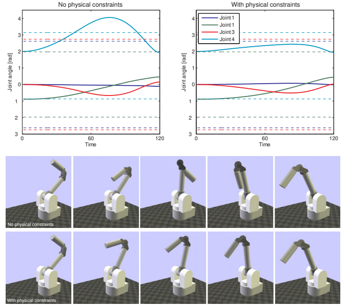
Fig. 4. Comparison of ILQG results obtained without (left) and with (right) physical constraint terms P(\mathbf{q}) and V(\dot{\mathbf{q}}) . The unconstrained solution violates the physical limits which would lead to a self collision applied to the WAM (top row of simulation screenshots).
