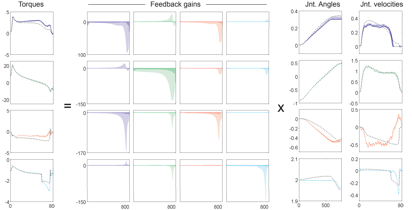
Fig. 5. Results of the ILQG control law (eq. 8) applied to the WAM with 4 DOF for a reaching to the center target \mathbf{t}_{center} . The dashed lines represent the optimal desired trajectories produced by ILQG, and the solid lines show the 10 trajectories recorded from the WAM. The shaded areas depict the feedback gain matrix ( L ), where brighter shadings indicate the position gains ( P ) and the darker areas depict the velocity-gains ( D ).
