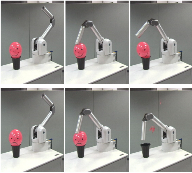
Fig. 7. Demonstration of the compliance of ILQG motion. Top row: The reaching with ILQG towards the center of the black bucket. The obstacle (balloon) cannot get damaged by the robot, due to the compliant motion of ILQG. In contrast the minimum jerk planning using standard gains is not compliant and therefore highly destructive.
