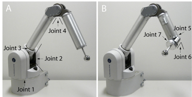
Fig. 1. The anthropomorphic manipulator (Barrett WAM) used for our experiments. (A): 4 DoF setup; (B): 7 DoF setup (with wrist attached).
