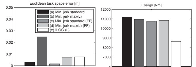
Fig. 6. Comparison of min jerk (conditions (1)-(4) and ILQG (5) - Results are averaged over 10 reaches to the center target ( \mathbf{t}_{center} ). Left: Euclidean distance (error) between target and end-point. Right: “Energy” consumption computed as sum of all torques in all joints over the entire trajectory: \sum_{i=1}^4 \sum_{k=1}^K |\mathbf{u}_k^{plant}(i)| .
