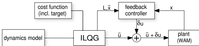
Fig. 2. The OFC scheme using ILQG.
