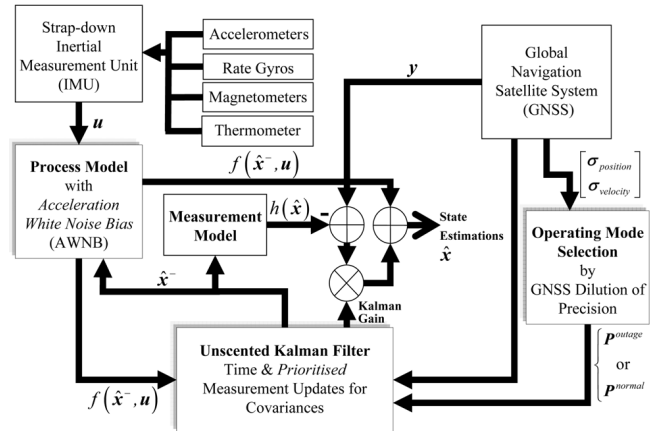
Fig. 8: The structure of the proposed state estimation algorithm.
