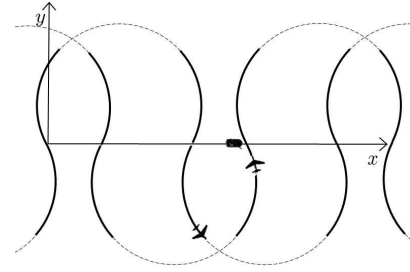
Fig. 6. Example of using two UAVs to provide continuous convoy protection using the proposed strategy. In this figure, the dashed curves are the paths of the UAVs, the solid curves are the segments of the paths in which convoy protection is provided. In this case, every time one UAV exits the convoy circle, the other UAV is inside the convoy circle. This is always true if N = \lceil \frac{\beta}{\gamma^*} \rceil = 2 and the times when the UAVs synchronize with the UGVs are spaced out.
