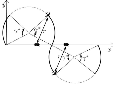
Fig. 5. For each execution of one motion primitive, there are two segments of the path corresponding to two circular arcs of angle \gamma^* , so that the distance between the UAV and the UGVs is less or equal to r when the UAV is on these segments. In this figure, the dashed curve is the path of the UAV, the solid curves are the segments of the path in which convoy protection is provided. The UAV and the convoys are drawn at the times when the UAV enters and exits these segments.
