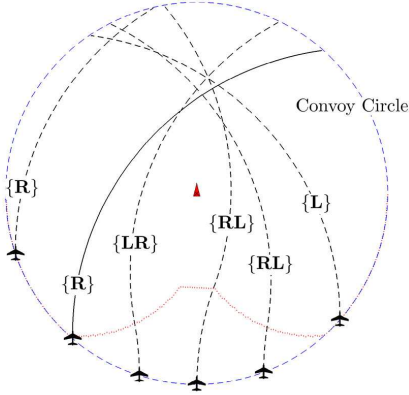
Fig. 2. A number of optimal state trajectories with initial heading \frac{\pi}{2} . The optimal switching points are plotted together to form the optimal switching surface. In this case, R = 1.5r . The dashed paths corresponds to optimal paths. The solid path corresponds to one initial position and this path is longer than all other optimal paths with the same initial heading.
