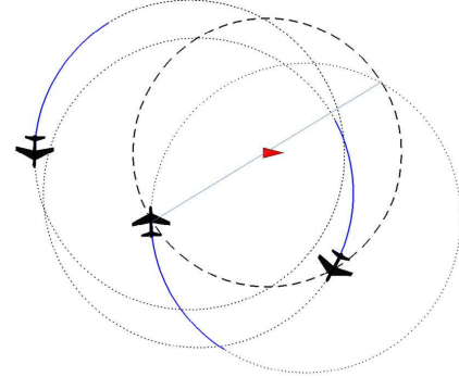
Fig. 3. Three optimal convoy protection paths are shown. They maximize the time spent inside the convoy circle over the time outside of the convoy circle. The smaller dashed circle is the convoy circle, and the larger dotted circles are optimal convoy protection paths. The solid circle is the past trajectories of the UAV.
