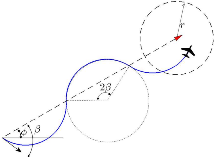
Fig. 4. Example trajectory of a UAV providing convoy protection for the UGVs with the proposed control strategy. The solid curve is the path of the UAV. The dashed line is the path of the UGVs. The dashed circle is the convoy circle. The angle of the circular arc for each motion primitive is 2\beta . In this case, \beta \in [0, \frac{\pi}{2}] .
