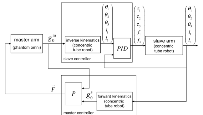
Fig. 5. Teleoperator block diagram.
