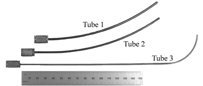
Fig. 4. Tubes comprising the robot. Tubes 1 and 2 form a variable curvature balanced pair that dominate tube 3. Ruler shows units in mm.
