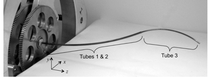
Fig. 3. Three-tube concentric tube robot.
