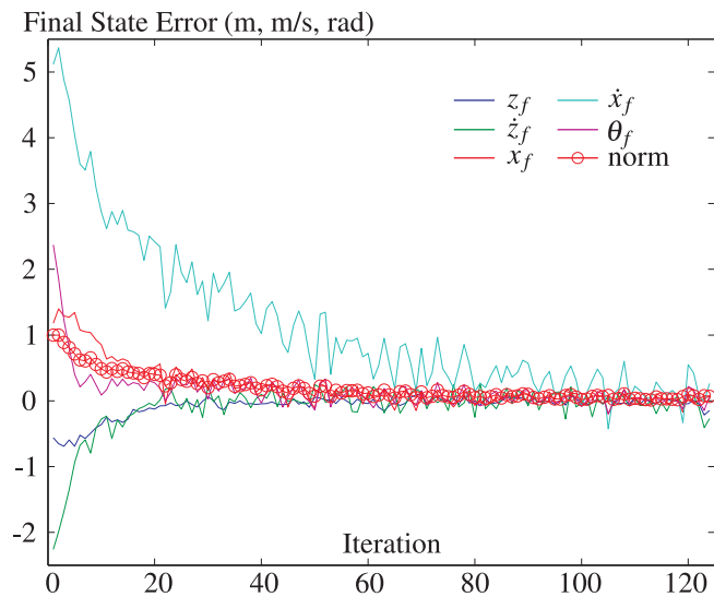
Fig. 11. Final state error and parameter evolution over 124 iterations for a vehicle with \dot{\theta}_{max} = 1300^\circ/s using \mathbf{J} and \mathbf{P}^0 calculated for \dot{\theta}_{max} = 1600^\circ/s . Step size \gamma = 0.07 . Note that \theta_f is normalized to (-\pi, \pi) .
