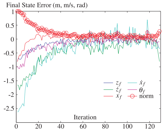
Fig. 9. Evolution of final state errors over a 129-iteration run of a 1600 ^{\circ}/s double flip. Step size \gamma was set to 0.1.
