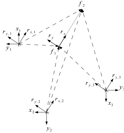
Fig. 3. Example of algorithm agreement on a common reference frame for a multi-agent system composed of three agents.
