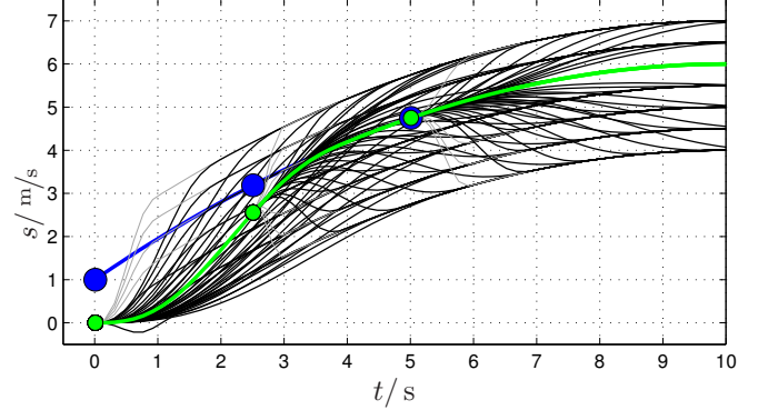
Fig. 4. Optimal longitudinal tracking of a target position in blue with green being the optimal trajectory, black the valid, and gray the invalid alternatives in each replanning step
