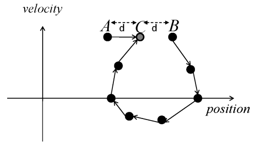
Fig. 3. Nodes A and B are equidistant to point C with respect to the Euclidean distance metric. However the children of node B, which has positive velocity, must be to the right of their parent, and therefore cannot get closer to C. In this case, Euclidean distance fails to distinguish between two nodes, one which is clearly the right choice for extending towards C, and the other which is not.
