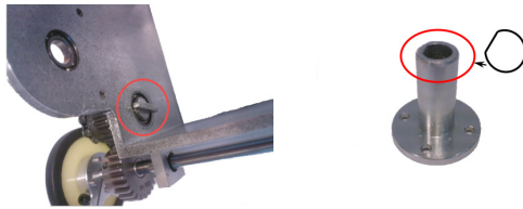
(a) Shaft locking mechanism. (b) Fork ear for shaft coupling.
