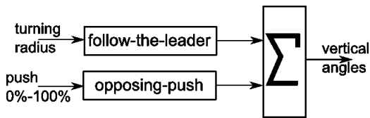
Fig. 16. Conceptual scheme for vertical motion.
