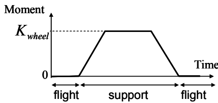
Fig. 8 Wheel moment
