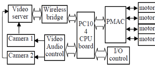
Fig2. Mobile vehicle control systems structure
