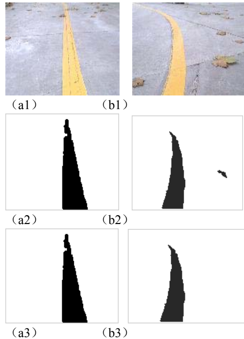
Fig.3 Image processing
