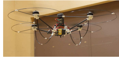
Fig. 1. Quad-rotor UAV used in our experiments
