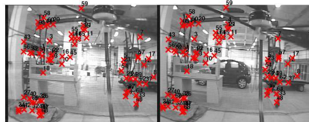
Fig. 10. Robustly matched features between the current image (left) and the image to reach (left; Im-6)
