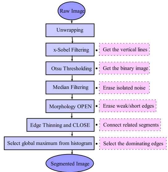
Fig. 4. The segmentation process
