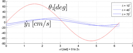
Fig. 5. The relation between \theta_1 and \dot{y}_1 for \alpha = 70^\circ , \omega = 70^\circ , and \delta = 10^\circ (dotted), 40^\circ (dashed), 70^\circ (solid).
