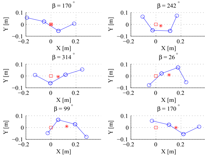
Fig. 9. The motion of the snake robot over one period of the cyclic locomotion.
