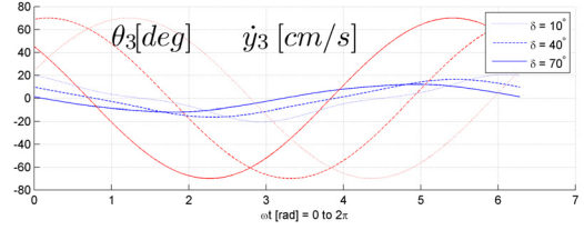
Fig. 7. The relation between \theta_3 and \dot{y}_3 for \alpha = 70^\circ , \omega = 70^\circ , and \delta = 10^\circ (dotted), 40^\circ (dashed), 70^\circ (solid).
