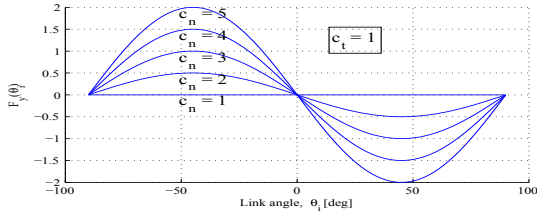
Fig. 4. The mapping from sideways link motion to forward propulsion for different viscous friction coefficients.
