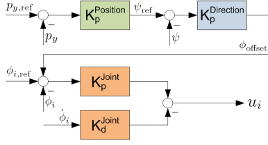
Fig. 8. The controller of the snake robot.
