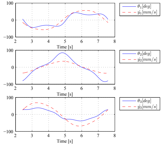
Fig. 11. Plot of \theta_i and \dot{y}_i ( i = 1, 2, 3 ) over one period of the cyclic locomotion.
