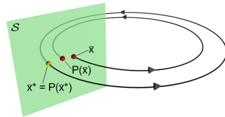
Fig. 1. Illustration of the Poincaré map corresponding to a Poincaré section \mathcal{S} .
