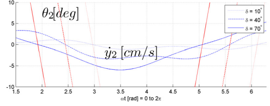
Fig. 6. The relation between \theta_2 and \dot{y}_2 for \alpha = 70^\circ , \omega = 70^\circ , and \delta = 10^\circ (dotted), 40^\circ (dashed), 70^\circ (solid). The plot is zoomed in.
