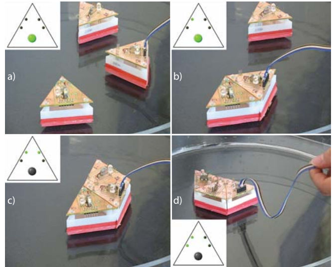
Fig. 8. Example for Tribolon state transition. The inset indicates the state as seen by the active module during the experiment, and its action (small circles: dark (no neighbor) and bright (connected neighbor); large circle: dark (motor stopped) and bright (motor running)): a) no neighbor: motor running, b) L: motor running, c) RL: motor stopped, d) LL: motor stopped. (see Fig. 6)
