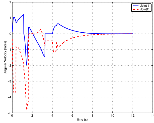
Fig. 6. Variation of the joint angle rates of the 2R robot for motion from start to goal configuration in Figure 5.
