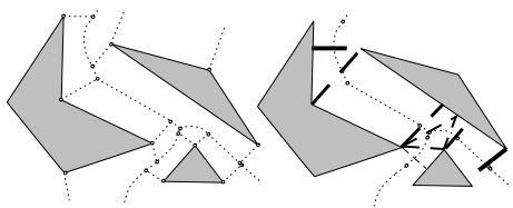
Fig. 3. Left: A Voronoi Diagram of the line segments of polygonal obstacles by considering each open segment and their endpoints as independent obstacles. Right: Conversion of the Voronoi Diagram into a surveillance graph. Dashed lines are associated to vertices and edges and represent blocks and sweeps. Thin lines move towards thicker lines.
