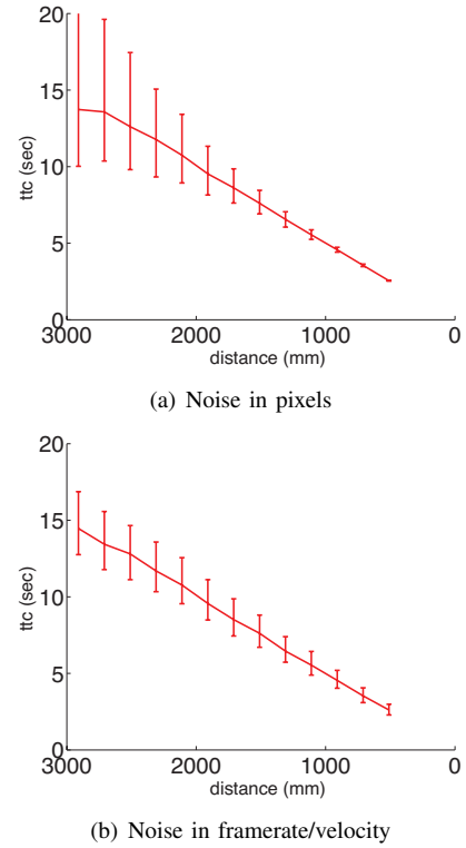
Fig. 2. Effect of noise in TTC estimation using a looming motion from 3000mm to 500mm. As expected the same level of induced noise has different effects on TTC depending on the remaining distance.
