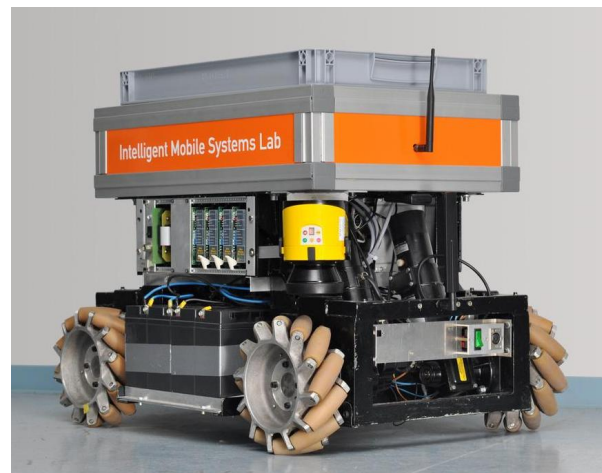
Fig. 1. Omnidirectional transport robot
