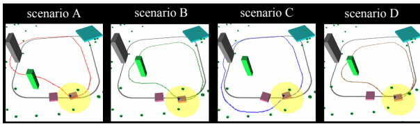
Fig. 3. Four obstacle scenarios designed for replaying the same taught path (black). Visual features are represented by the green points, the range scanner by a yellow disk, and the replayed paths are drawn in red (scenario A), green (B), blue (C), and brown (D).
